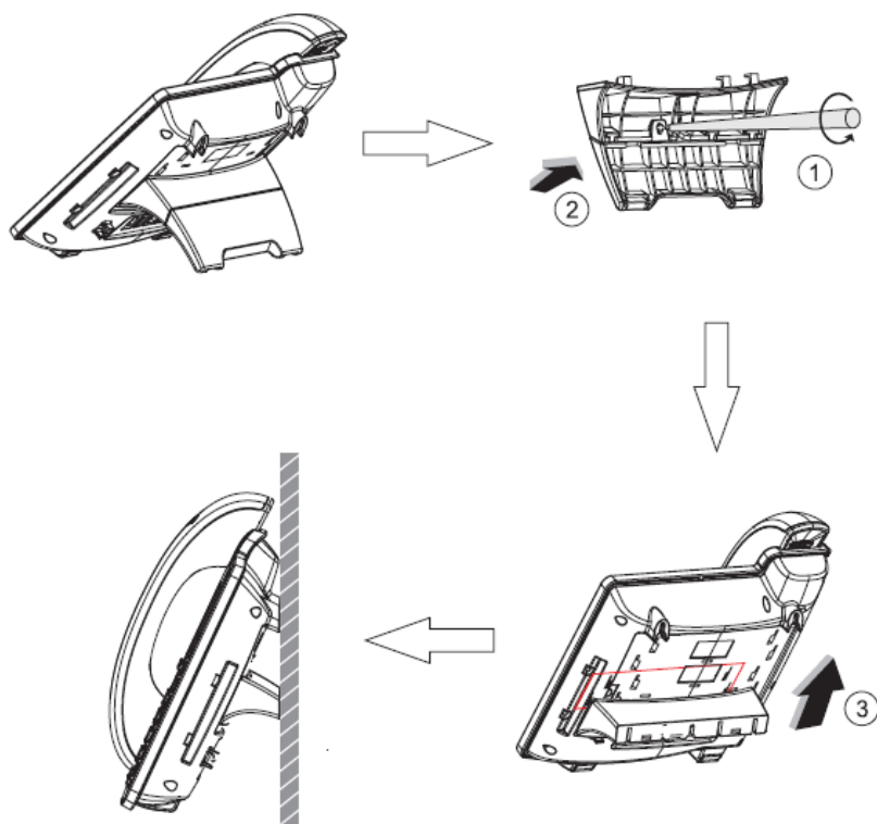
Figure 2 - Wall-mount Installation
